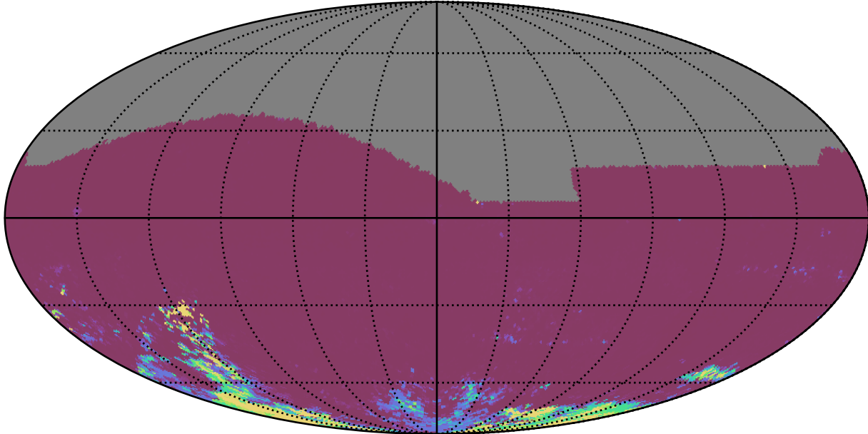
ddf_acor_sf10_lsf40_lsr20_v3.4_10yrs All sky ri bands: 75th Percentile Intranight Timespan
