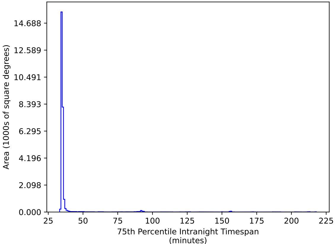
ddf_acor_sf10_lsf40_lsr20_v3.4_10yrs All sky ri bands: 75th Percentile Intranight Timespan
