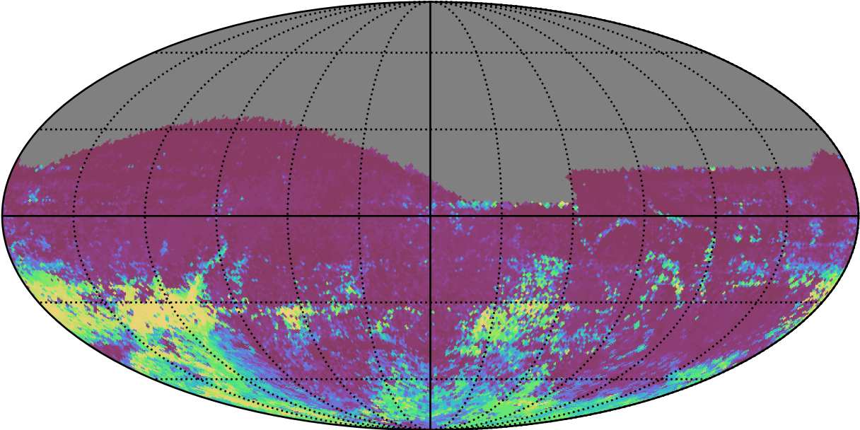
ddf_acor_sf10_lsf40_lsr20_v3.4_10yrs All sky r band: 75th Percentile Intranight Timespan
