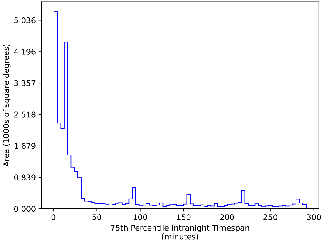
ddf_acor_sf10_lsf40_lsr20_v3.4_10yrs All sky r band: 75th Percentile Intranight Timespan
