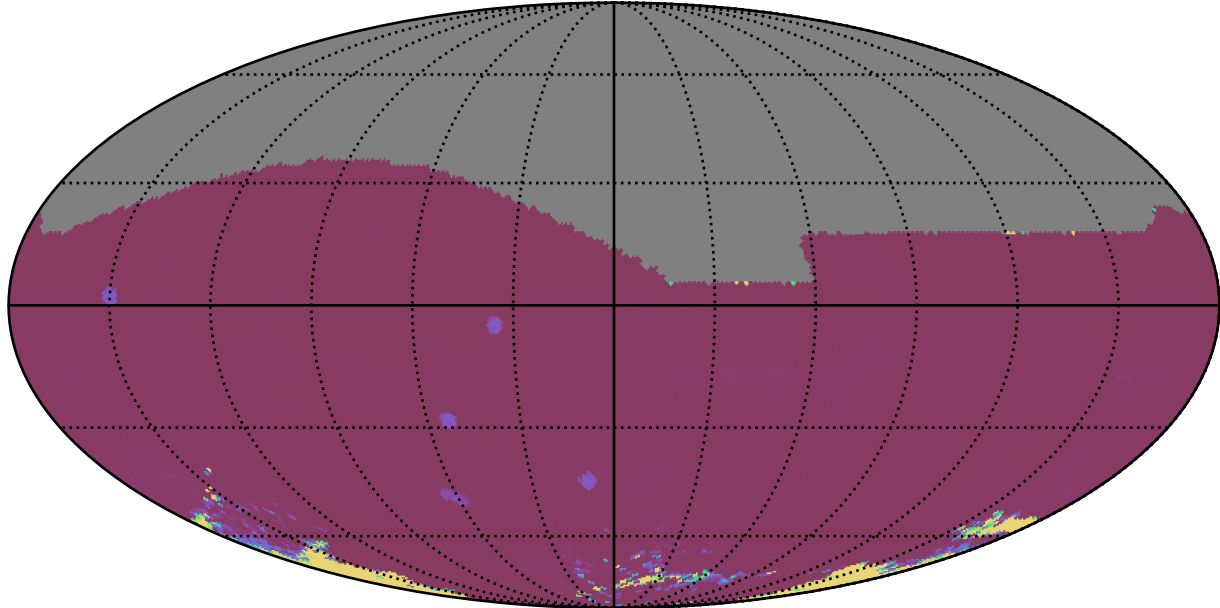
ddf_acor_sf10_lsf40_lsr20_v3.4_10yrs All sky iz bands: 75th Percentile Intranight Timespan
