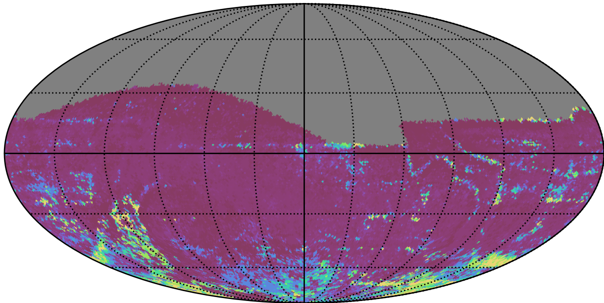
ddf_acor_sf10_lsf40_lsr20_v3.4_10yrs All sky i band: 75th Percentile Intranight Timespan
