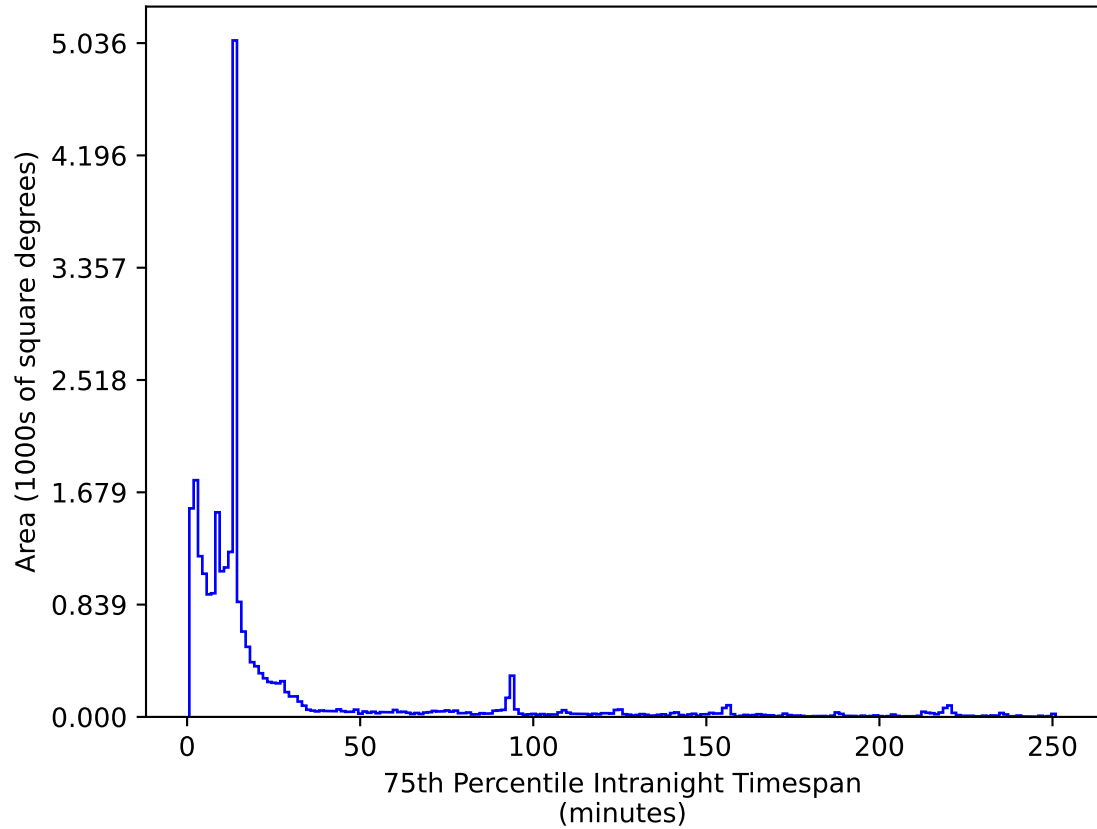
ddf_acor_sf10_lsf40_lsr20_v3.4_10yrs All sky i band: 75th Percentile Intranight Timespan
