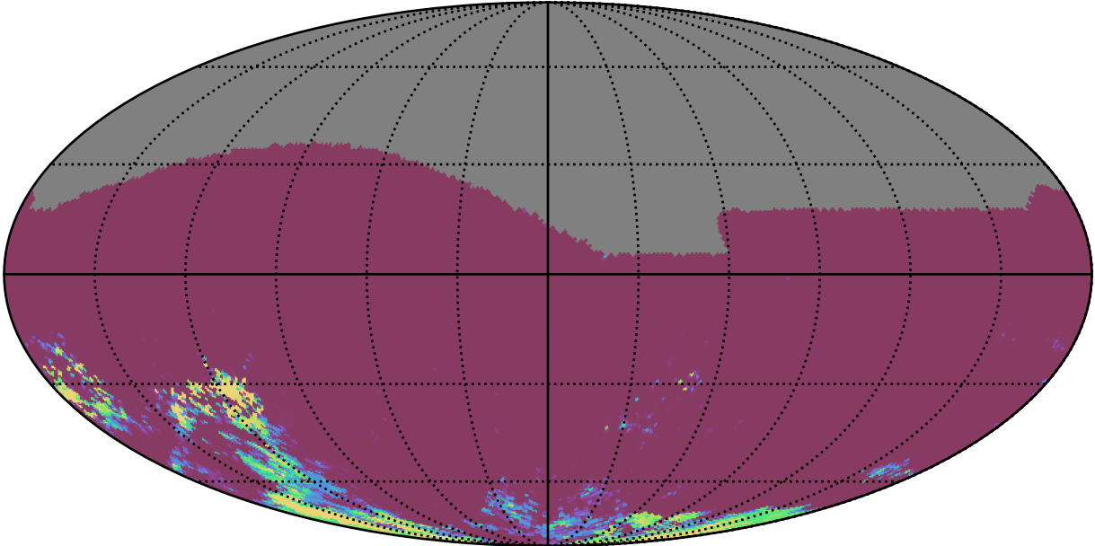
ddf_acor_sf10_lsf40_lsr20_v3.4_10yrs All sky gr bands: 75th Percentile Intranight Timespan
