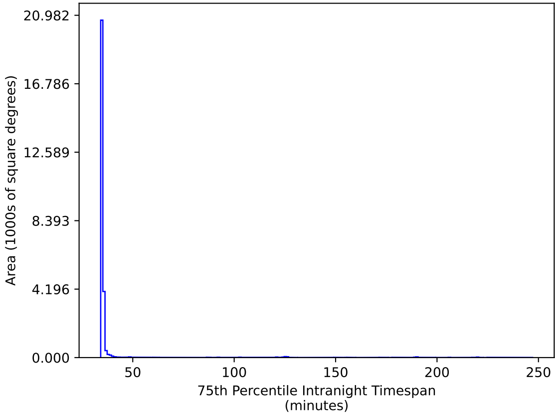
ddf_acor_sf10_lsf40_lsr20_v3.4_10yrs All sky gr bands: 75th Percentile Intranight Timespan
