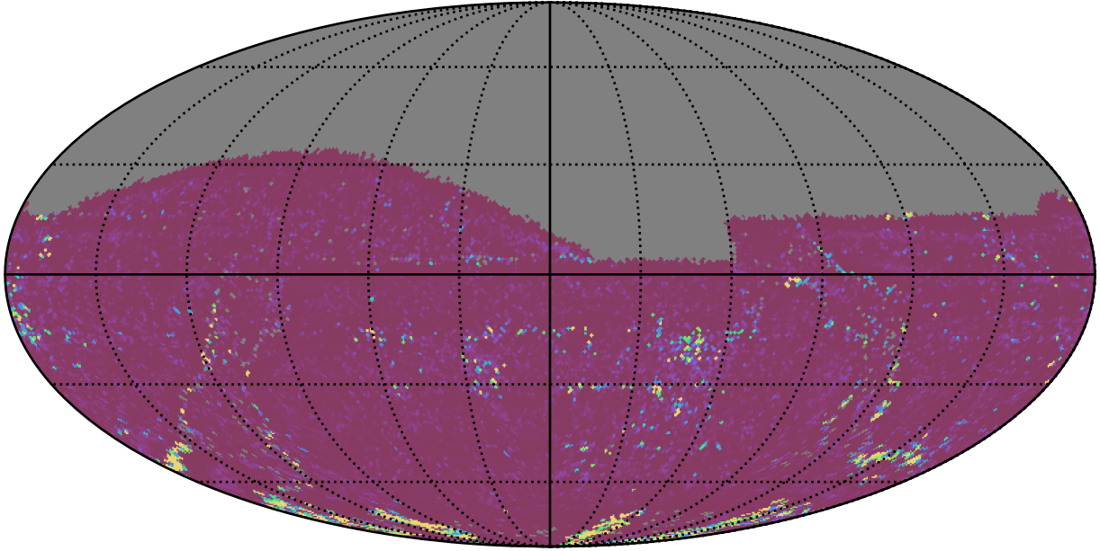
ddf_acor_sf10_lsf40_lsr20_v3.4_10yrs All sky g band: 75th Percentile Intranight Timespan
