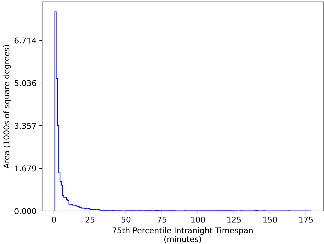
ddf_acor_sf10_lsf40_lsr20_v3.4_10yrs All sky g band: 75th Percentile Intranight Timespan
