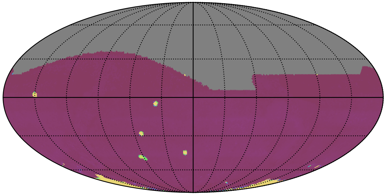
ddf_acor_sf10_lsf40_lsr20_v3.4_10yrs All sky: 75th Percentile Intranight Timespan
