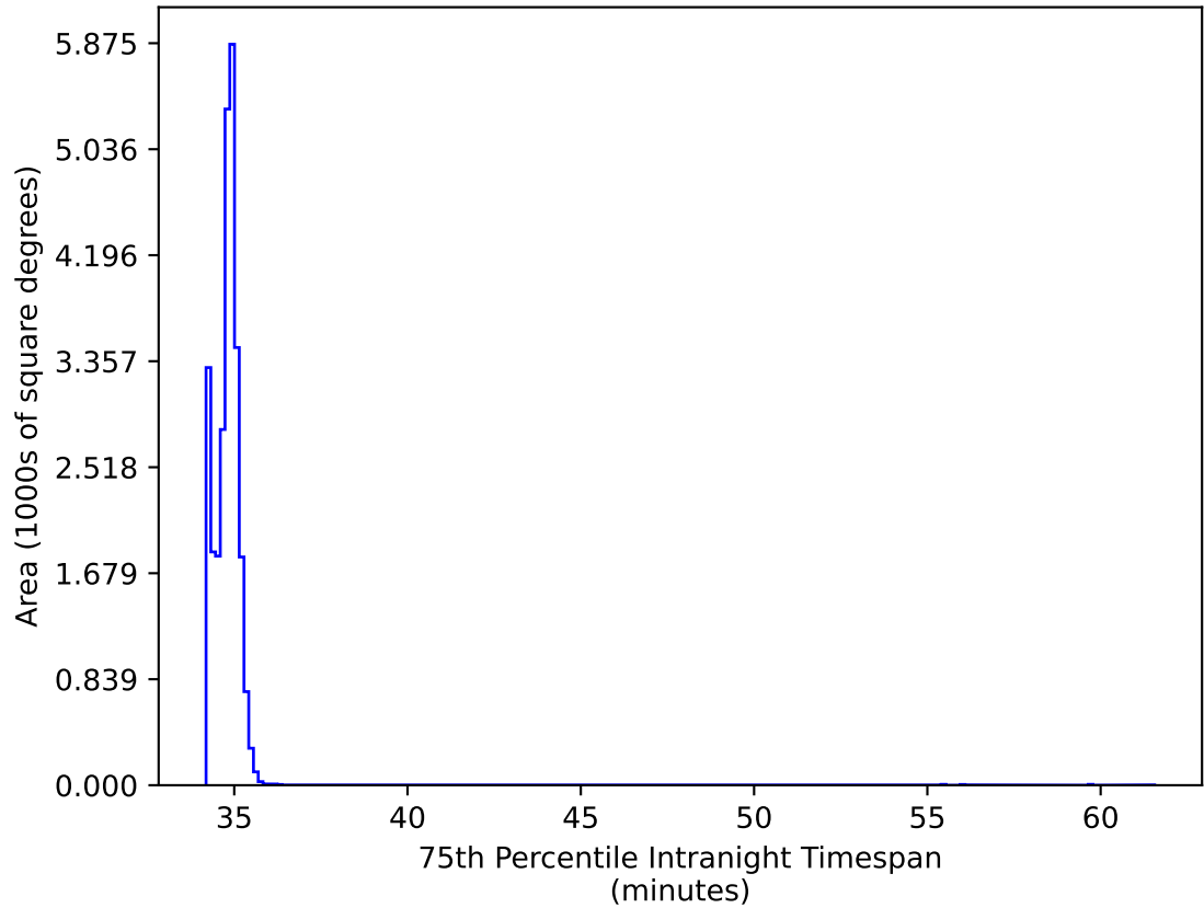
ddf_acor_sf10_lsf40_lsr20_v3.4_10yrs All sky: 75th Percentile Intranight Timespan
