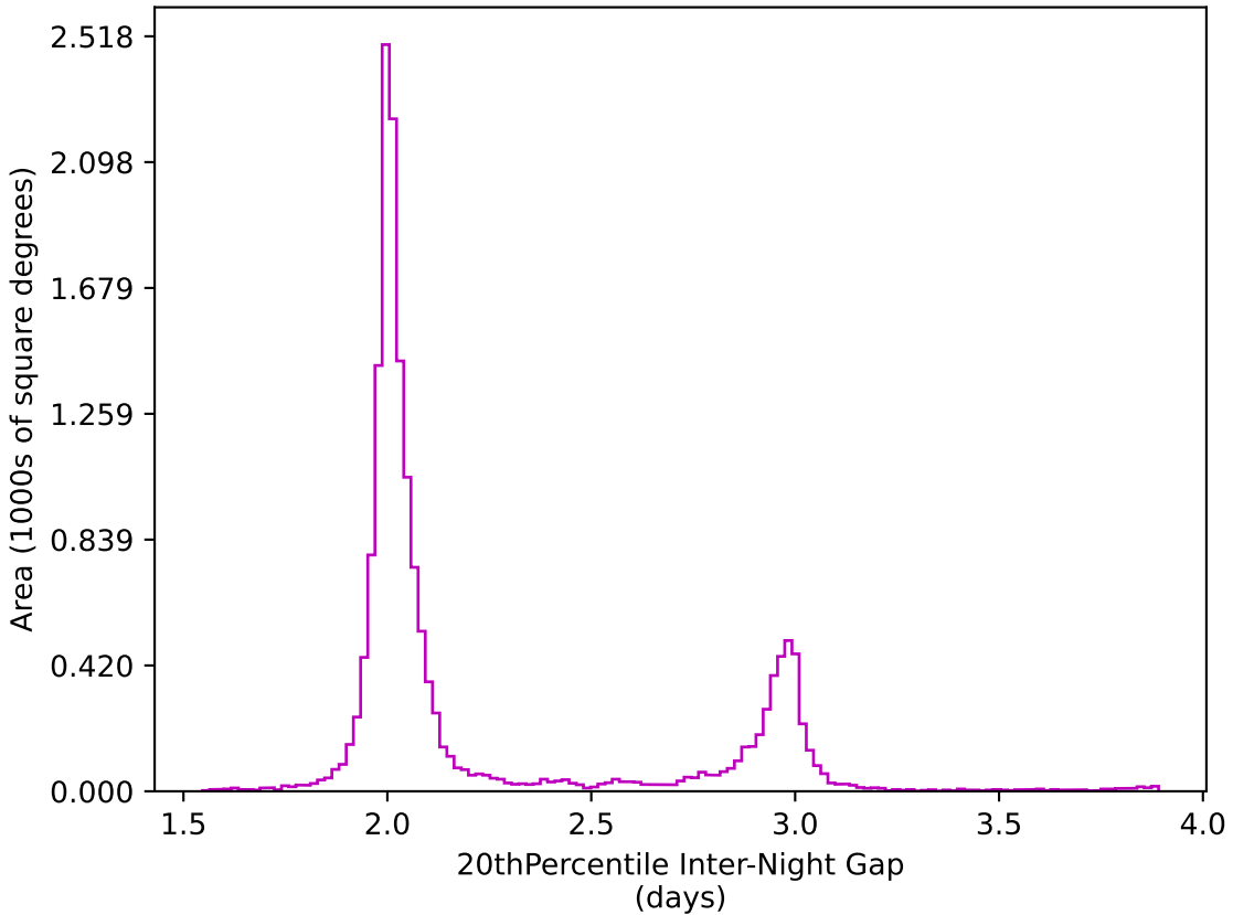
ddf_acor_sf10_lsf40_lsr20_v3.4_10yrs WFD z band: 20thPercentile Inter-Night Gap
