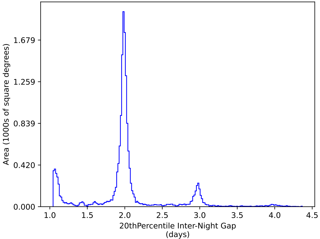
ddf_acor_sf10_lsf40_lsr20_v3.4_10yrs WFD y band: 20thPercentile Inter-Night Gap
