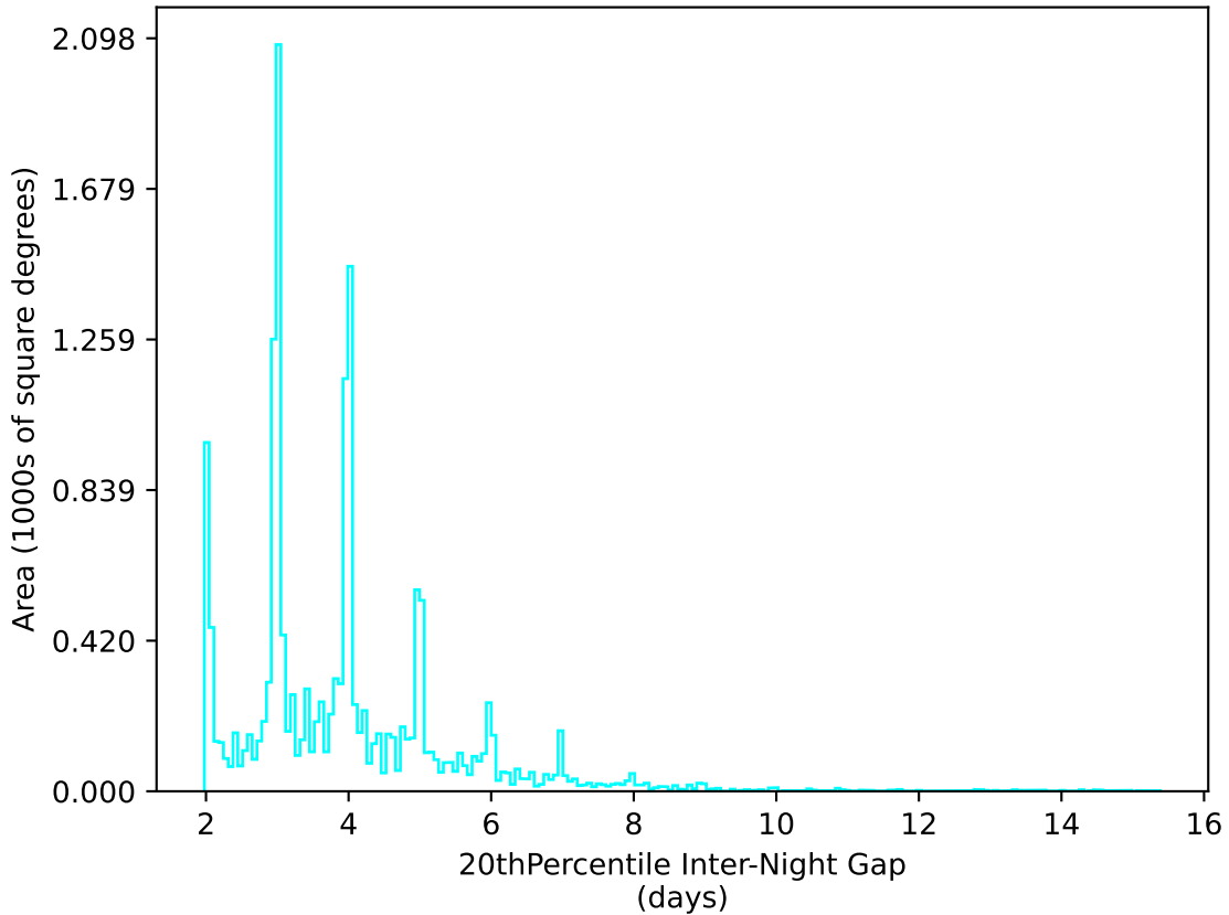
ddf_acor_sf10_lsf40_lsr20_v3.4_10yrs WFD u band: 20thPercentile Inter-Night Gap
