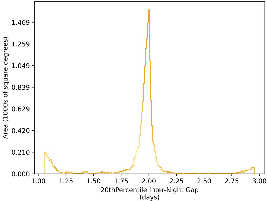
ddf_acor_sf10_lsf40_lsr20_v3.4_10yrs WFD r band: 20thPercentile Inter-Night Gap
