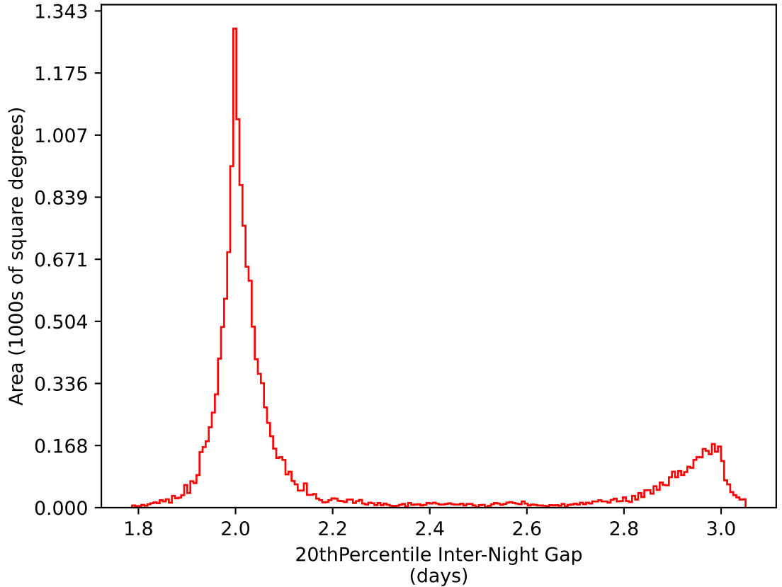
ddf_acor_sf10_lsf40_lsr20_v3.4_10yrs WFD i band: 20thPercentile Inter-Night Gap
