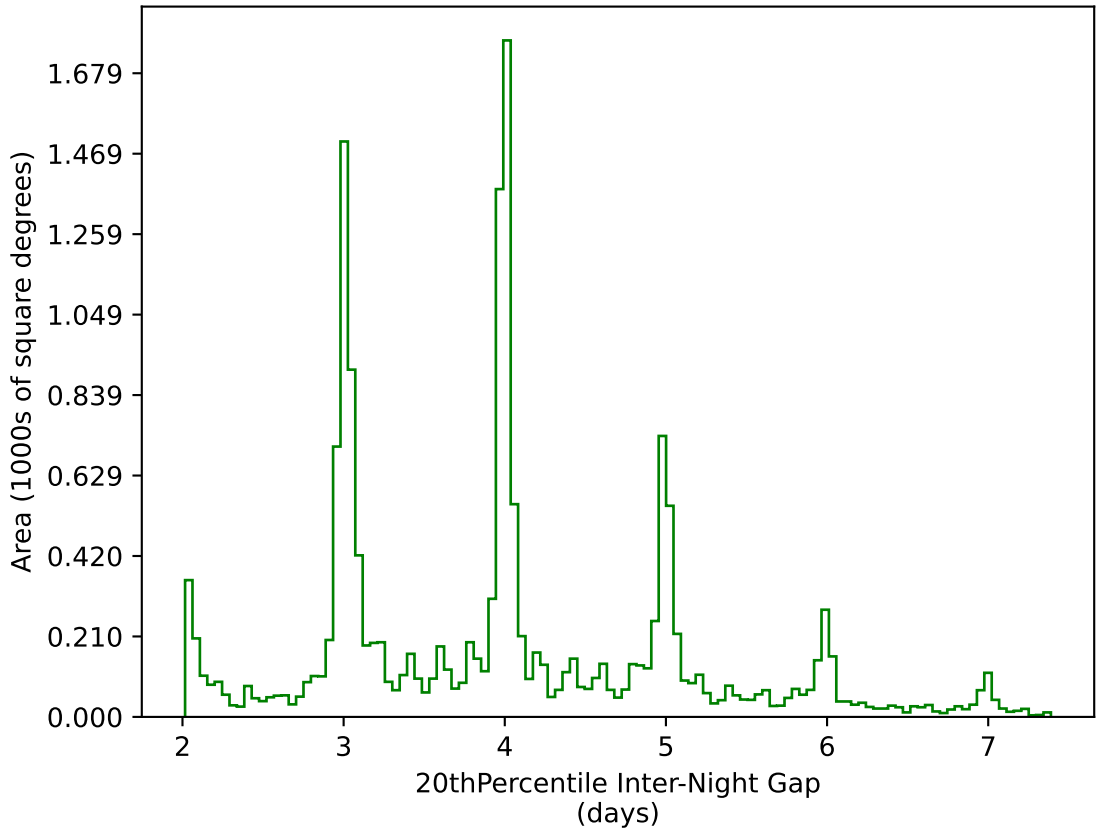
ddf_acor_sf10_ls40_lsr20_v3.4_10yrs WFD g band: 20thPercentile Inter-Night Gap
