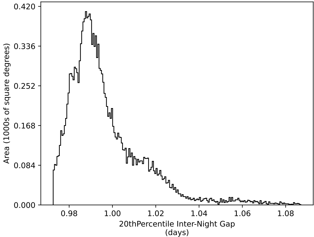
ddf_acor_sf10_lsf40_lsr20_v3.4_10yrs WFD all bands: 20thPercentile Inter-Night Gap
