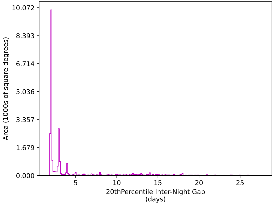
ddf_acor_sf10_ls40_lsr20_v3.4_10yrs All sky z band: 20thPercentile Inter-Night Gap
