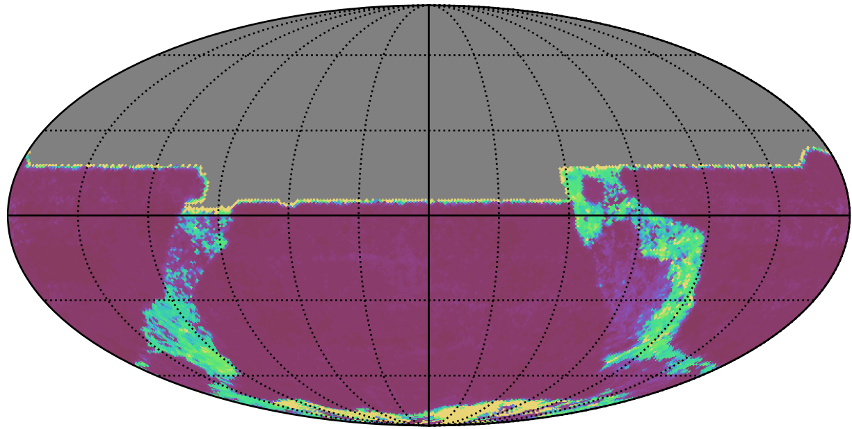
ddf_acor_sf10_lsf40_lsr20_v3.4_10yrs All sky y band: 20thPercentile Inter-Night Gap
