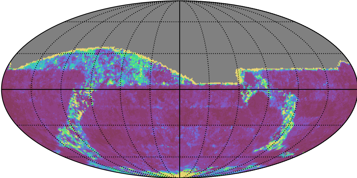
ddf_acor_sf10_lsf40_lsr20_v3.4_10yrs All sky g band: 20thPercentile Inter-Night Gap
