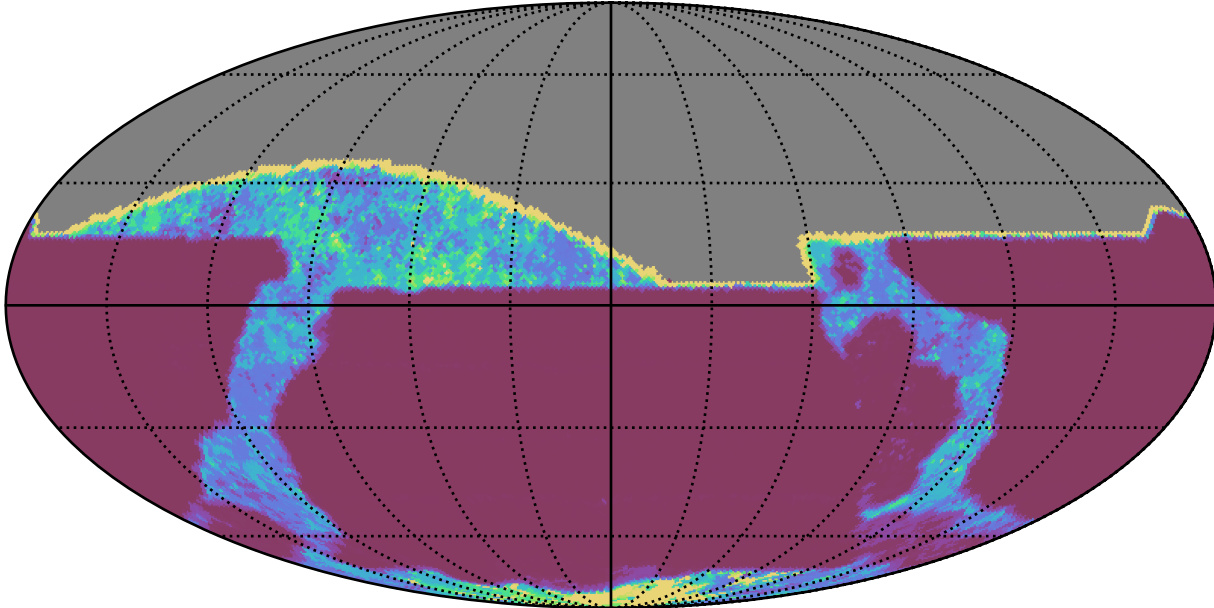
ddf_acor_sf10_lsf40_lsr20_v3.4_10yrs All sky all bands: 20thPercentile Inter-Night Gap
