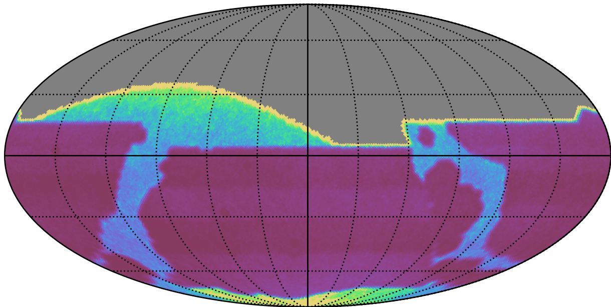
ddf_acor_sf10_lsf40_lsr20_v3.4_10yrs : properMotion
