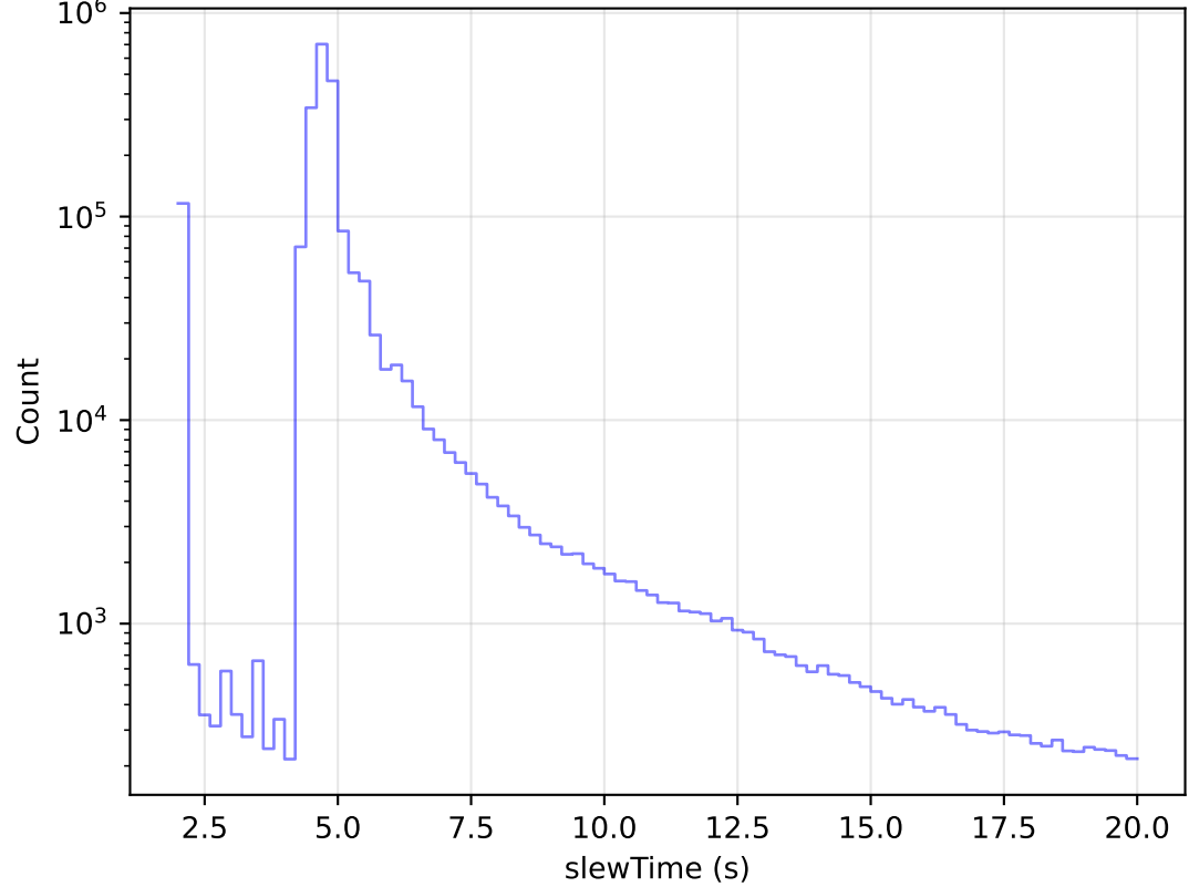
ddf_acor_sf10_Isf40_Isr20_v3.4_10yrs All visits: Zoom Slew Time Histogram
