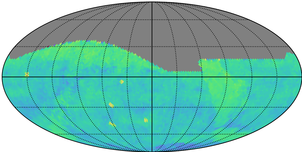
ddf_acor_sf10_lsf40_lsr20_v3.4_10yrs (g or r or i): PairFraction
