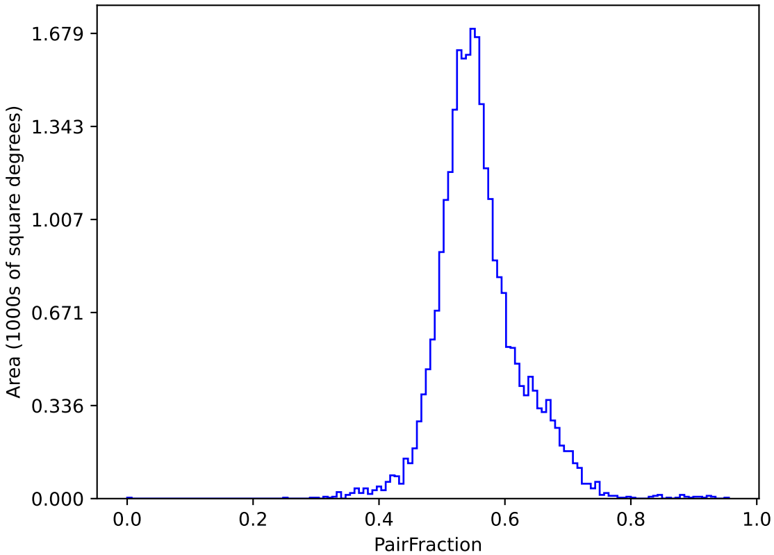
ddf_acor_sf10_lsf40_lsr20_v3.4_10yrs (g or r or i): PairFraction
