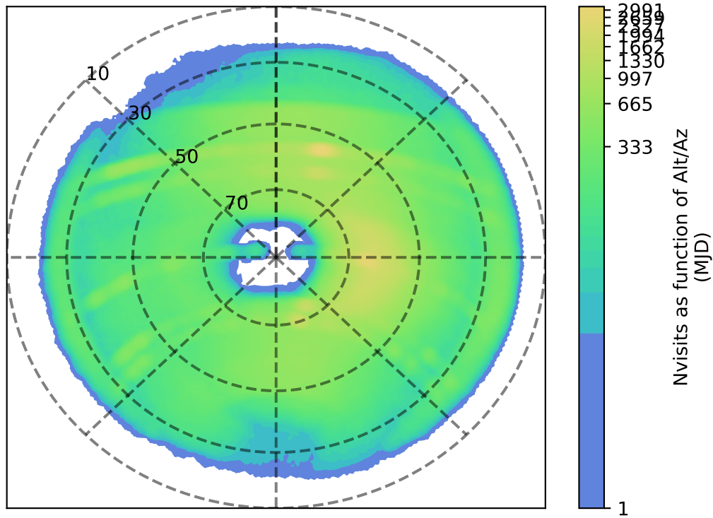
ddf_acor_sf10_lsf40_lsr20_v3.4_10yrs z: Nvisits as function of Alt/Az
