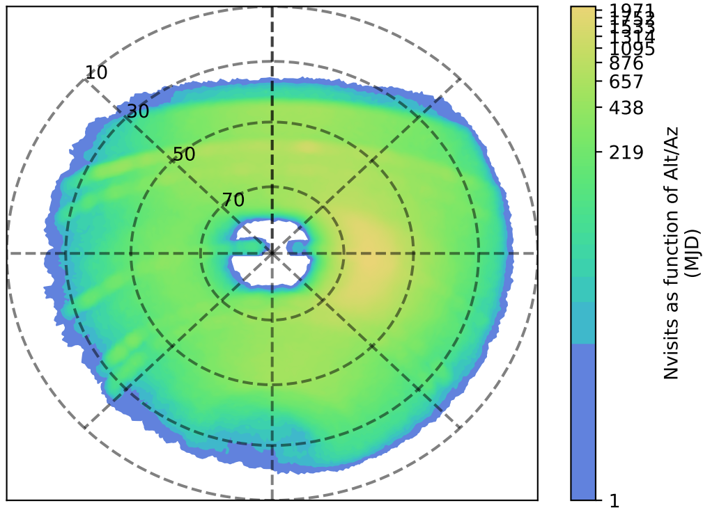
ddf_acor_sf10_lsf40_lsr20_v3.4_10yrs y: Nvisits as function of Alt/Az
