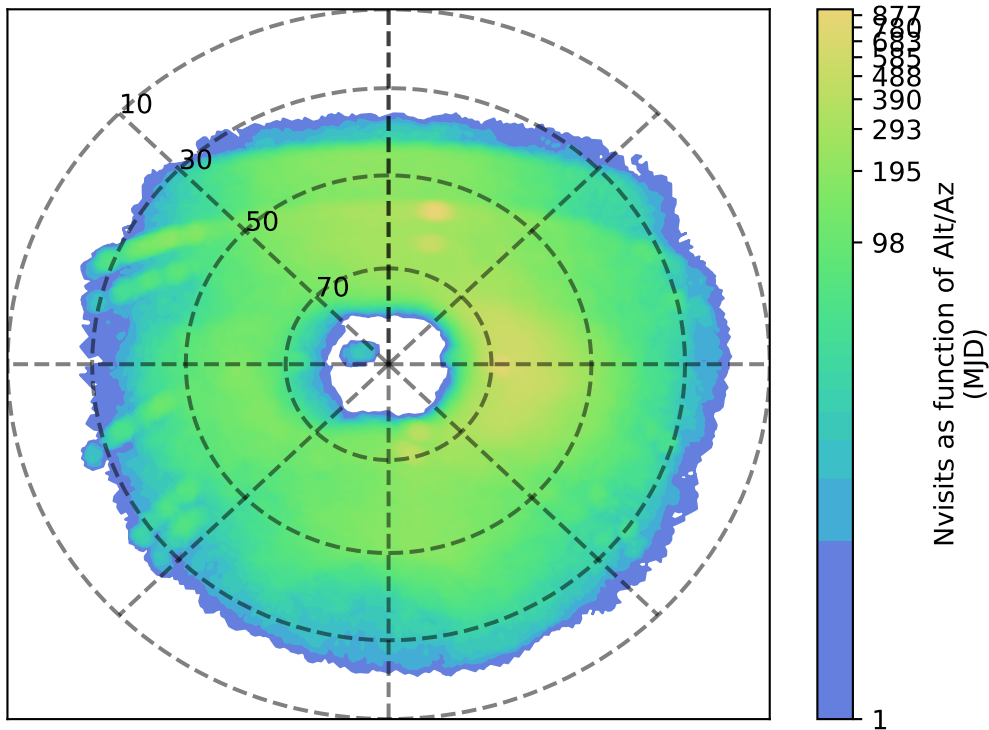
ddf_acor_sf10_lsf40_lsr20_v3.4_10yrs u: Nvisits as function of Alt/Az
