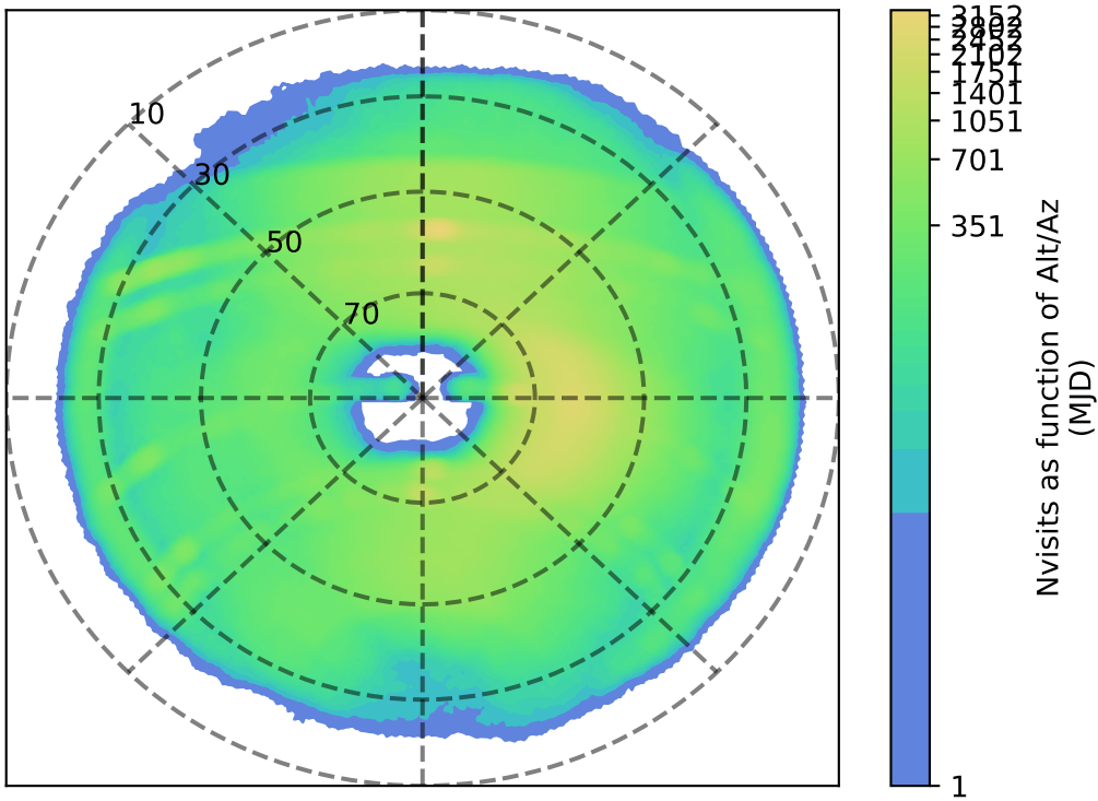
ddf_acor_sf10_ls40_lsr20_v3.4_10yrs i: Nvisits as function of Alt/Az
