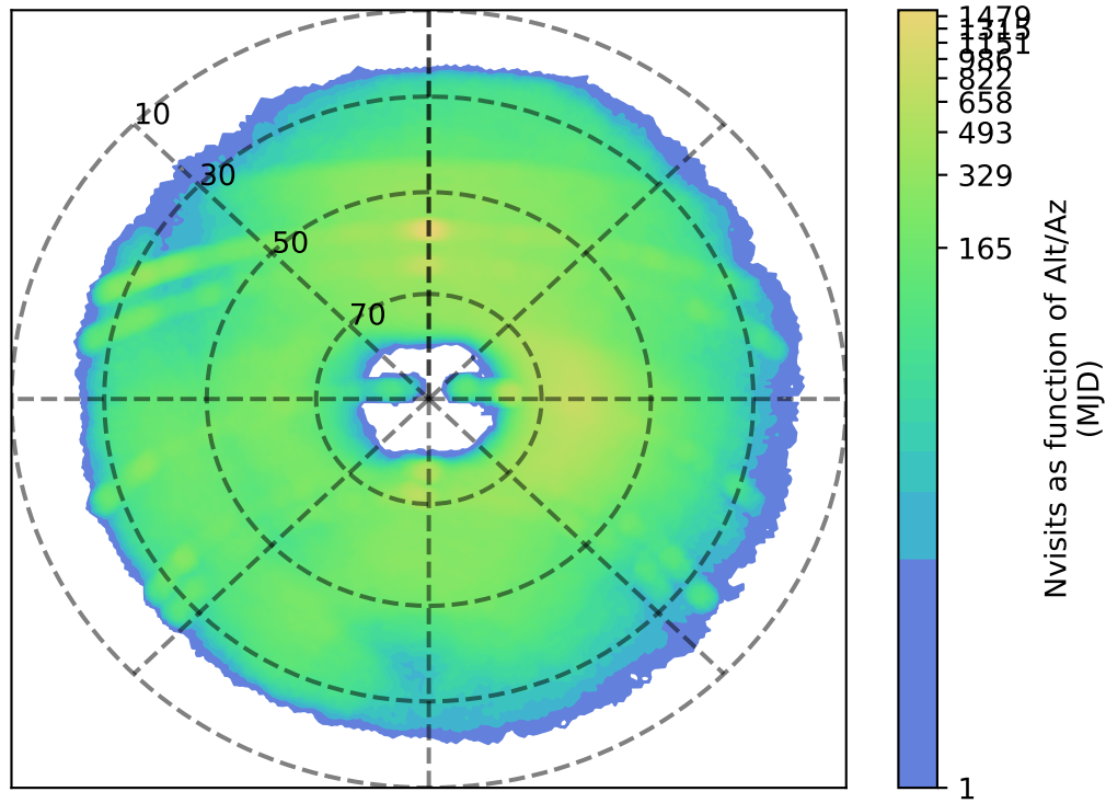
ddf_acor_sf10_lsf40_lsr20_v3.4_10yrs g: Nvisits as function of Alt/Az
