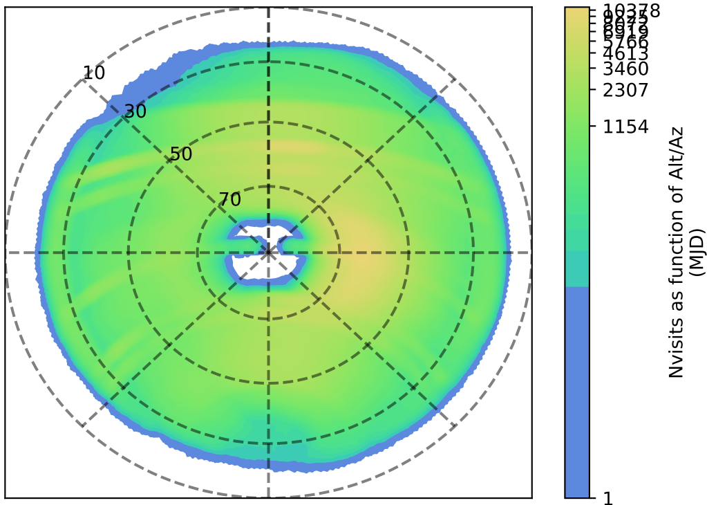
ddf_acor_sf10_lsf40_lsr20_v3.4_10yrs : Nvisits as function of Alt/Az
