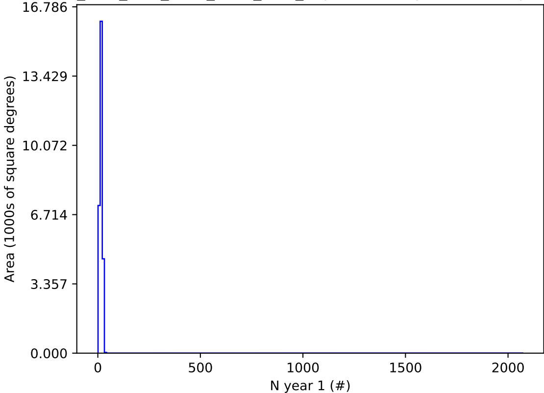
ddf_acor_sf10_lsf40_lsr20_v3.4_10yrs r and night < 365: N year 1
