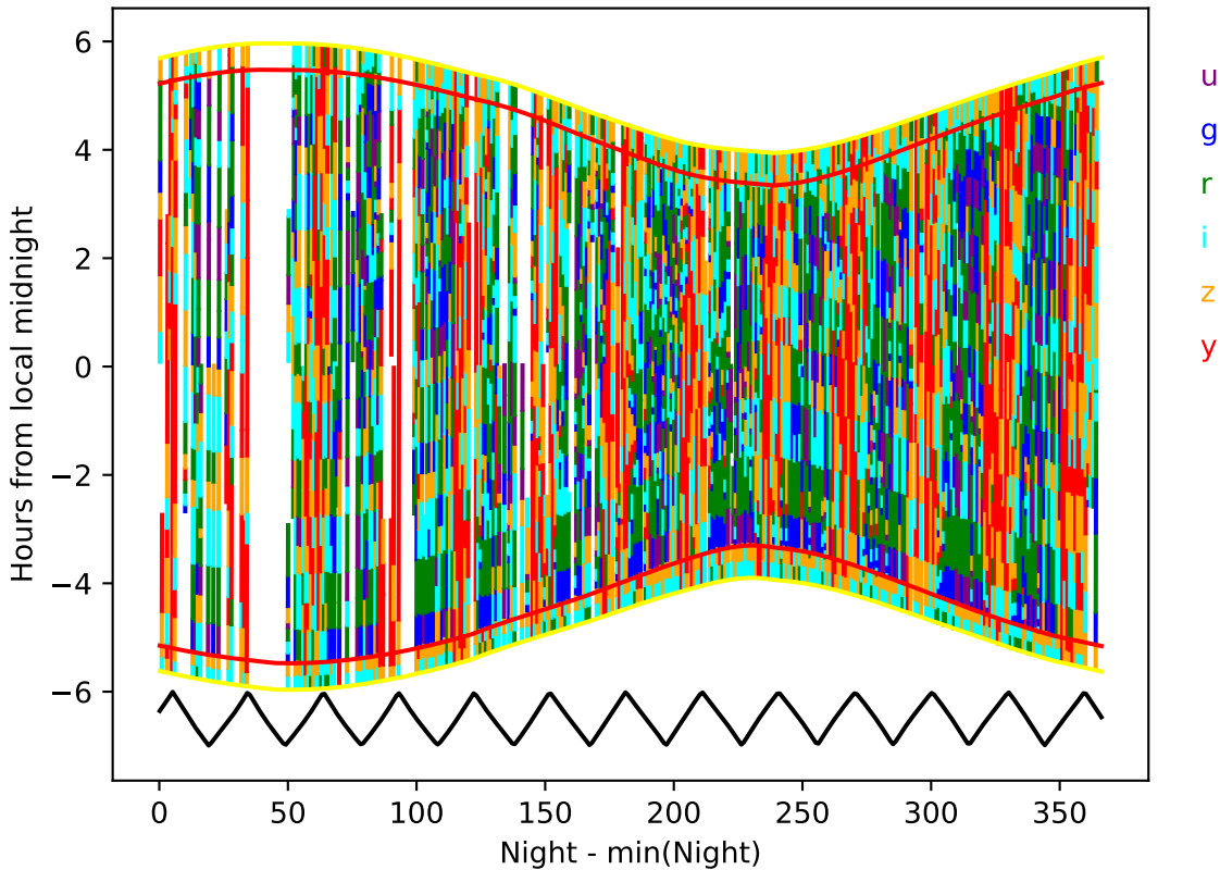
ddf_acor_sf10_lsf40_lsr20_v3.4_10yrs year 6-7: Hourglass
