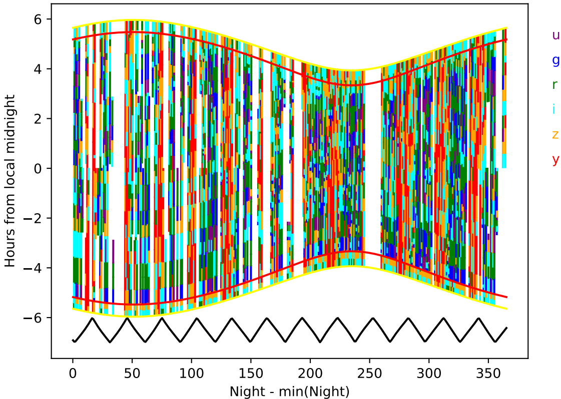
ddf_acor_sf10_ls40_lsr20_v3.4_10yrs year 5-6: Hourglass
