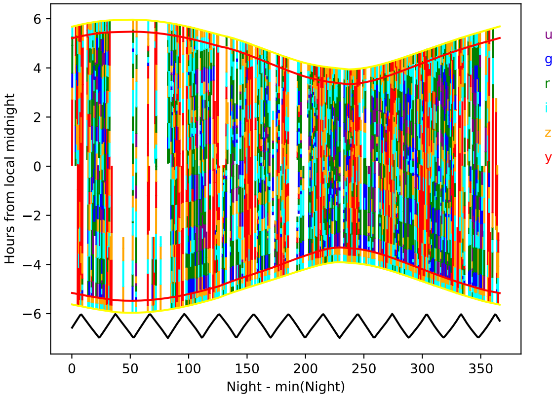
ddf_acor_sf10_lsf40_lsr20_v3.4_10yrs year 3-4: Hourglass
