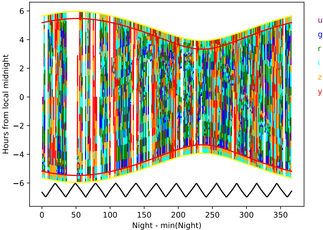
ddf_acor_sf10_lsf40_lsr20_v3.4_10yrs year 2-3: Hourglass
