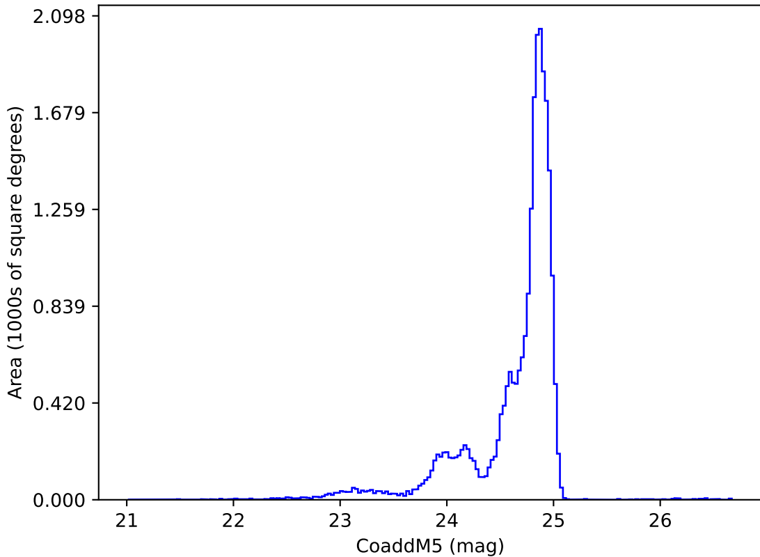
ddf_acor_sf10_lsf40_lsr20_v3.4_10yrs y: CoaddM5
