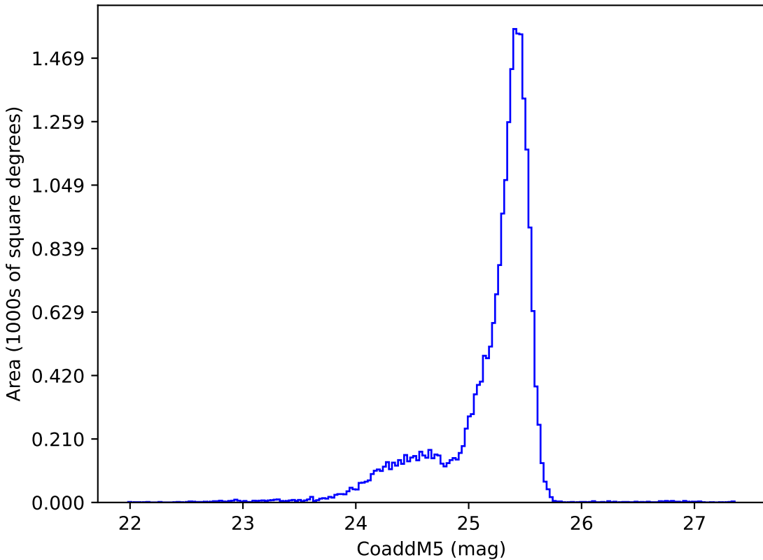
ddf_acor_sf10_ls40_lsr20_v3.4_10yrs u: CoaddM5
