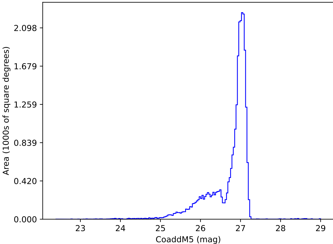
ddf_acor_sf10_lsf40_lsr20_v3.4_10yrs r: CoaddM5
