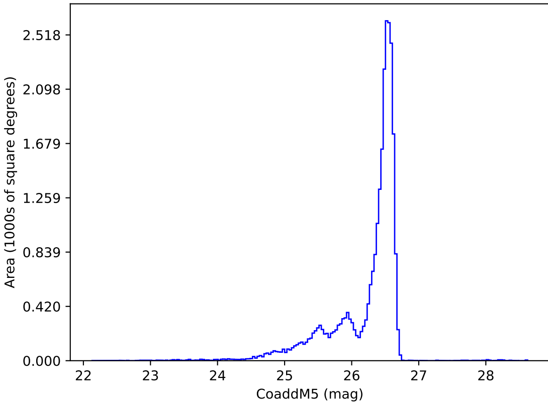
ddf_acor_sf10_lsf40_lsr20_v3.4_10yrs i: CoaddM5
