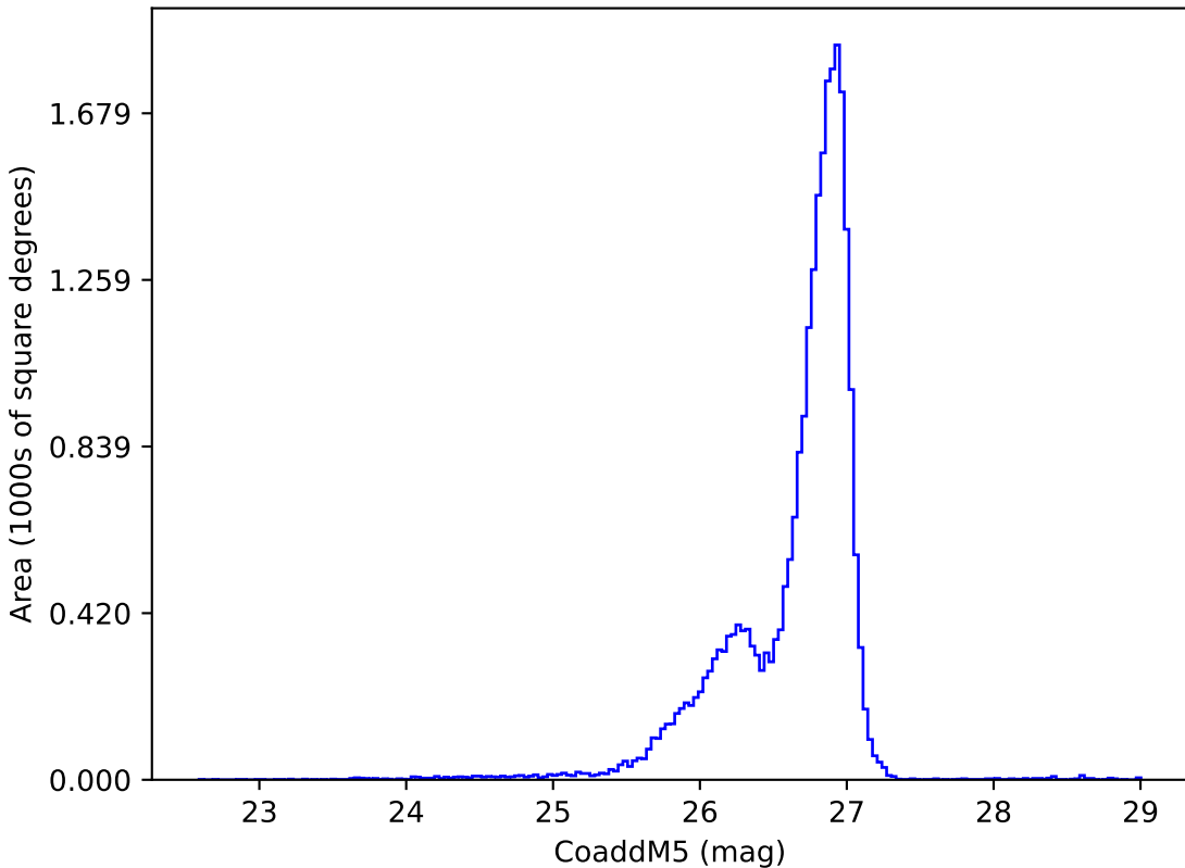
ddf_acor_sf10_lsf40_lsr20_v3.4_10yrs g: CoaddM5
