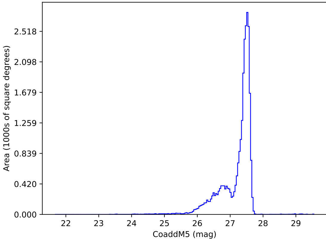
ddf_acor_sf10_lsf40_lsr20_v3.4_10yrs : CoaddM5
