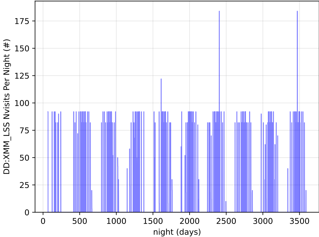
ddf_acor_sf10_lsf40_lsr20_v3.4_10yrs all bands: DD:XMM_LSS Nvisits Per Night
