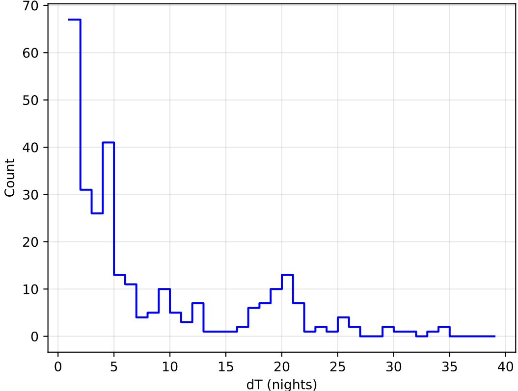
ddf_acor_sf10_Isf40_Isr20_v3.4_10yrs all bands: DD:XMM_LSS Delta Nights Histogram
