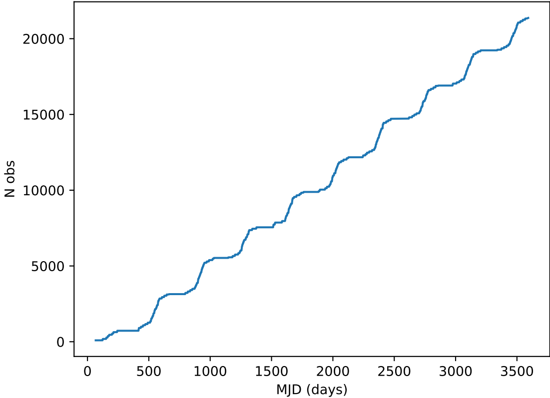
ddf_acor_sf10_lsf40_lsr20_v3.4_10yrs all bands: DD:XMM_LSS Cumulative NVisits
