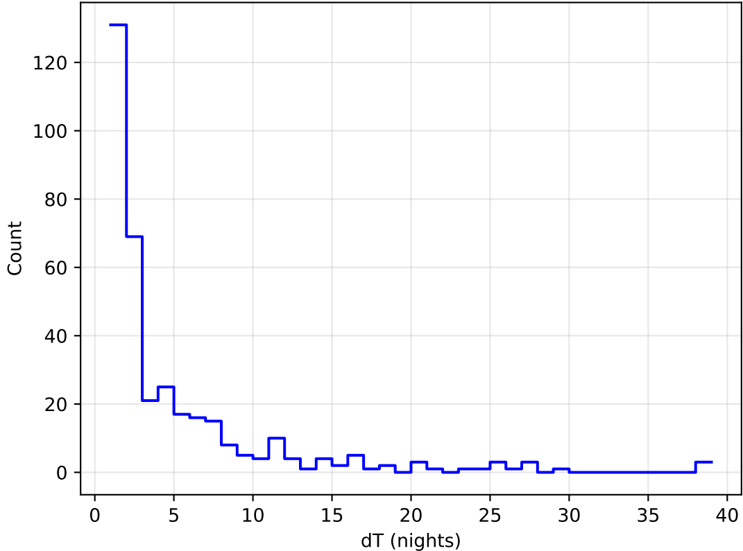
ddf_acor_sf10_lsf40_lsr20_v3.4_10yrs all bands: DD:WFD Delta Nights Histogram
