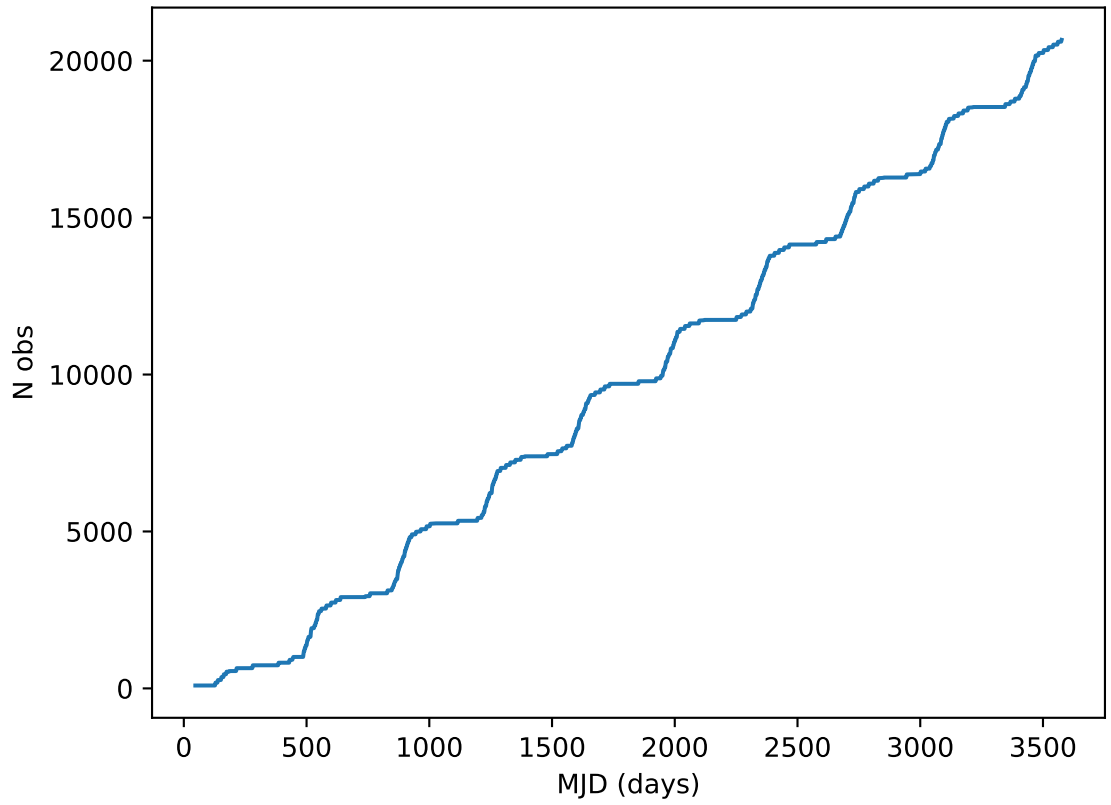
ddf_acor_sf10_lsf40_lsr20_v3.4_10yrs all bands: DD:ELAISS1 Cumulative NVisits
